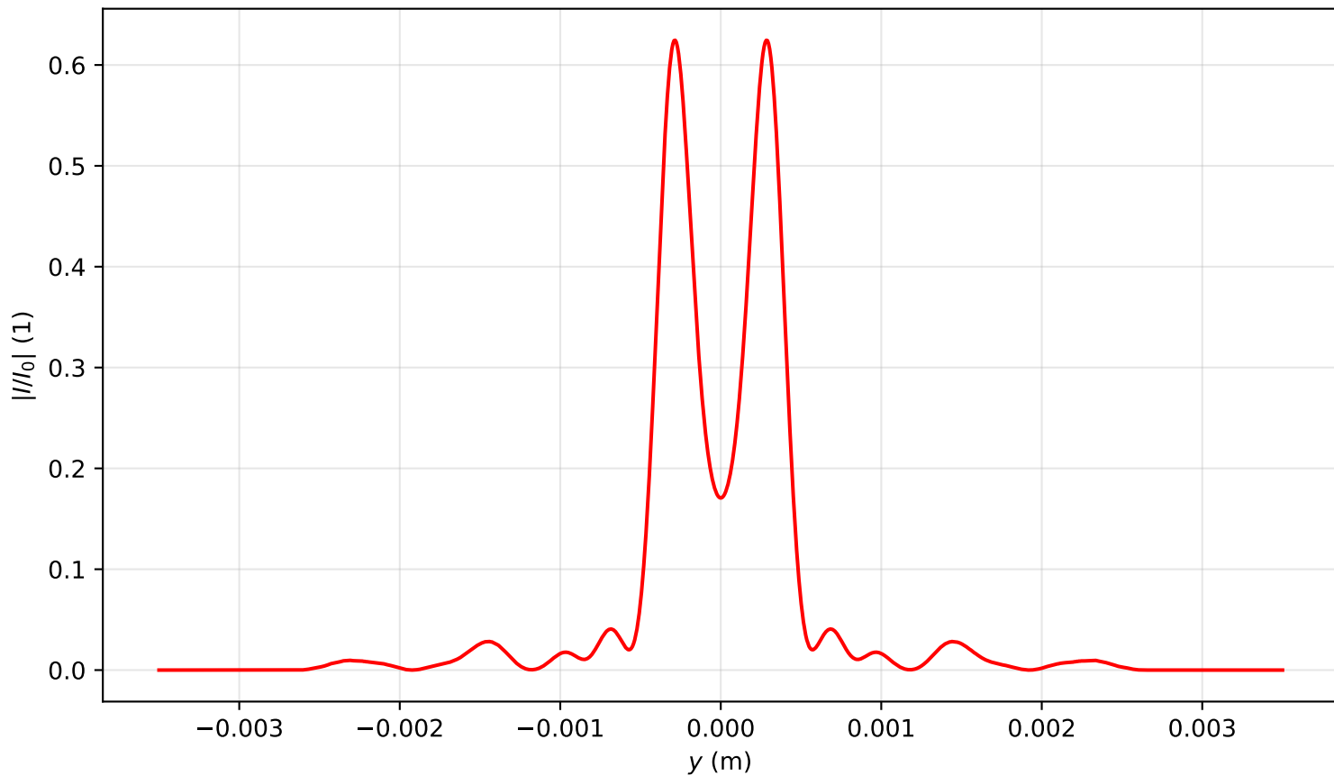
Intensity profile I(x=0, y, z=0.637)/I_0 , \text{Pin}=3.0\text{Pcr} , artificial time
